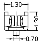
C-C SEC
