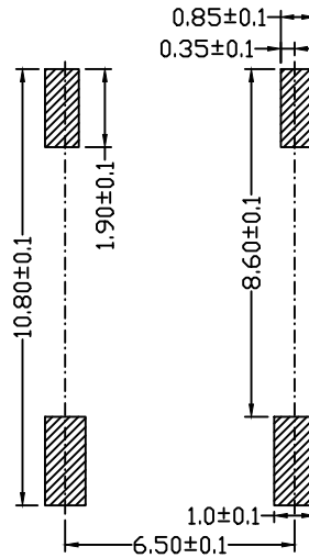
Recommand PCB Layout
