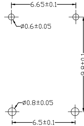
Recommened PCB Layout
