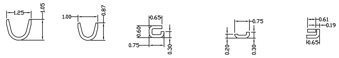
Section: A-A Section: B-B Section: C-C Section: D-D Section: E-E
