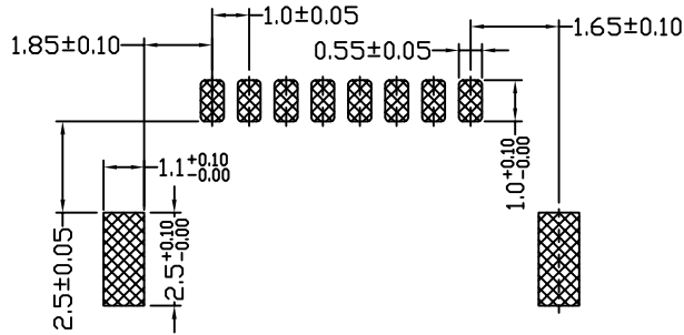
Recommant PCB Layout
